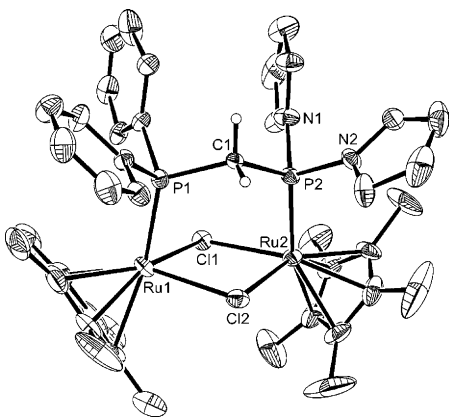
Figure 8. Molecular structure of [\text{Ru}_2\text{Cp}^*_2(\mu\text{-Cl})_2(\mu\text{-L})] 8 with the phenyl, pyrrolyl, and methyl protons omitted for clarity and thermal ellipsoids shown at the 30% probability level.
