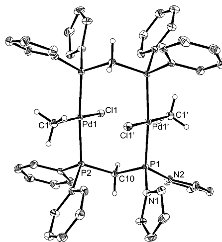
Figure 6. Molecular structure of [\text{Pd}_2\text{Cl}_2(\text{CH}_3)_2(\mu\text{-L})_2] 6 with the phenyl and pyrrolyl protons omitted for clarity and thermal ellipsoids shown at the 30% probability level.
