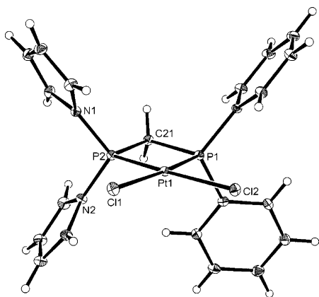
Figure 2. Molecular structure of [\text{PtCl}_2(\text{L-}\kappa^2\text{P,P}')]\cdot\text{CH}_2\text{Cl}_2 ( 3 · \text{CH}_2\text{Cl}_2 ) with the included solvent omitted for clarity and thermal ellipsoids shown at the 30% probability level.
