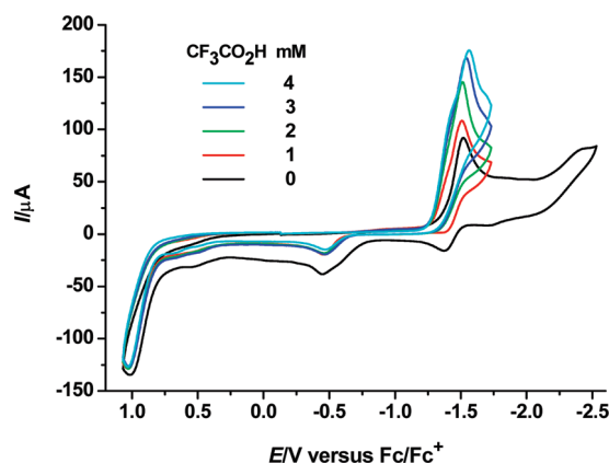
Figure 10. Cyclic voltammograms of 8 (1.0 mM) with CF 3 CO 2 H (0–4 mM) in 0.1 M n -Bu 4 NPF 6 /MeCN at a scan rate of 100 mV s −1 .
