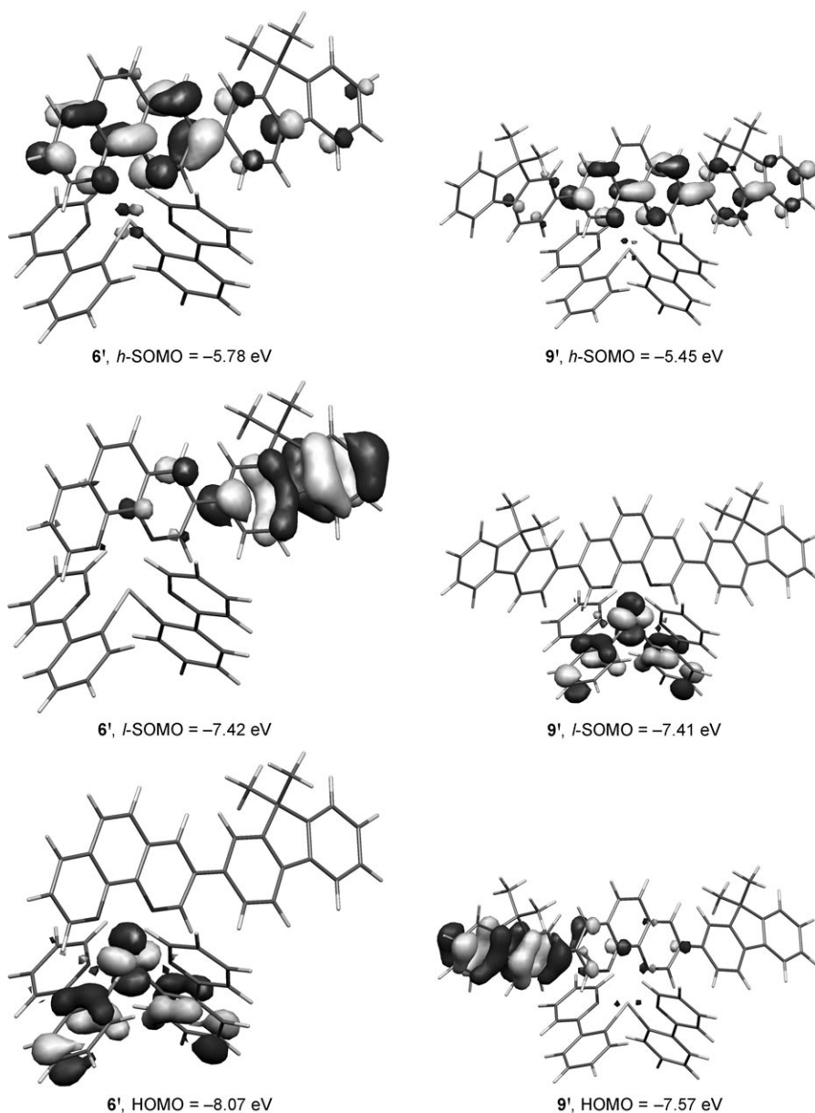
Figure 7. Isocontours plots ( 0.04 \text{ ebohr}^{-3} ) of higher and lower singly occupied molecular orbitals ( h -SOMO and I -SOMO) and HOMO ( \alpha electrons) orbitals for T_1 equilibrium geometries of complexes 6' and 9' .
