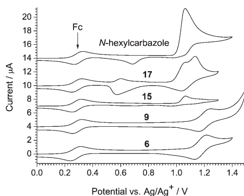
Figure 2. Cyclic voltammograms of complexes 6 , 9 , 15 , 17 and N -hexylcarbazole in a solution of 0.1 M Bu 4 NPF 6 dichloromethane, scan rate 100 mV s −1 , with ferrocene (Fc) as an internal reference.
