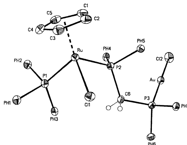
Figure 2. Thermal ellipsoids drawing of the molecular structure of \text{CpRu}(\text{PPh}_3)\text{Cl}(\mu\text{-dppm})\text{AuCl} ( 2 ). Thermal ellipsoids are plotted at 50% probability. Phenyl rings and most hydrogen atoms are omitted for clarity.
