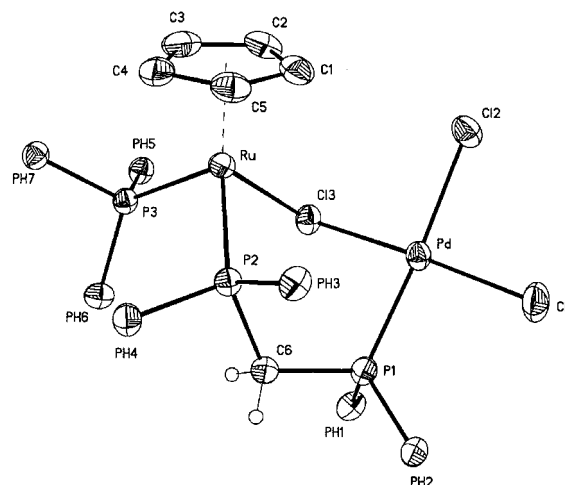
Figure 1. Thermal ellipsoids drawing of the molecular structure of \text{CpRu}(\text{PPh}_3)(\mu\text{-Cl})(\mu\text{-dppm})\text{PdCl}_2 ( 1 ). Thermal ellipsoids are plotted at 50% probability. Phenyl rings and most hydrogen atoms are omitted for clarity.
