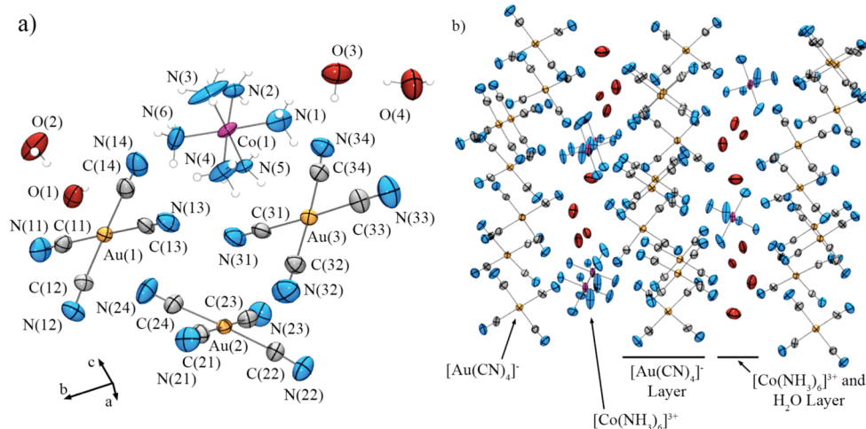
Figure 4. (a) Asymmetric unit of [\text{Co}(\text{NH}_3)_6][\text{Au}(\text{CN})_4]_3 \cdot 4\text{H}_2\text{O} (8) and (b) a view of the packing in the crystal structure, while looking down the a -axis, showing layers of [\text{Au}(\text{CN})_4]^- anions alternating with layers of [\text{Co}(\text{NH}_3)_6]^{3+} cations and water molecules. Hydrogen atoms in b are removed for clarity.
