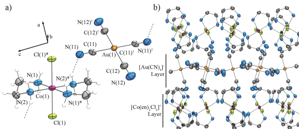
Figure 1. (a) Asymmetric unit of 6 showing the chain formed by hydrogen bonding between N(11)⋯H(21)*–N(2)* and (b) the view of the solid state crystal viewed down the a -axis showing layering that occurs between [ trans -Co(en) 2 Cl 2 ] + and [Au(CN) 4 ] − ions. Hydrogen atoms are removed for clarity.
