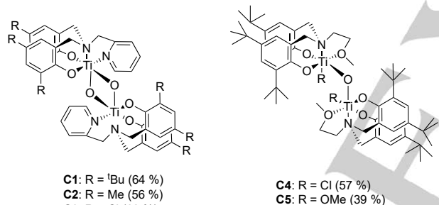
Figure 2. Structures of bimetallic Ti-O-Ti complexes ( C1 – C5 ).
