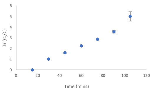
Figure 7. \alpha -Terpinene \ln(C_0/C) vs. time using complex C5 .
