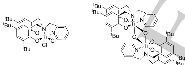
Figure 8. Structures of monometallic vs. bimetallic Ti complexes of ligand L1H2 .
