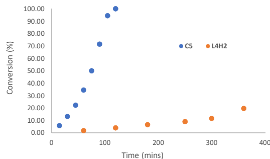
Figure 9. \alpha -Terpinene conversion in the presence of C5 vs. L4H2 .
