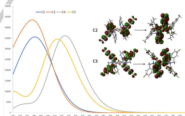
Figure 10. (TD)-CAM-B3LYP calculated absorption spectra for target molecules C2 – C5 . Inset are dominant particle-hole transitions for C2 and C3 highlighting the nature of the bright electronic states for each species through LMCT \pi to d\pi^* transitions. Spectra generated by convoluting a Gaussian (FWHM=20 nm) over lowest 30 singlet states.
