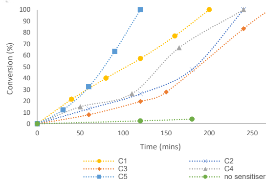
Figure 6. Conversion of \alpha -terpinene to ascaridole vs. time.
