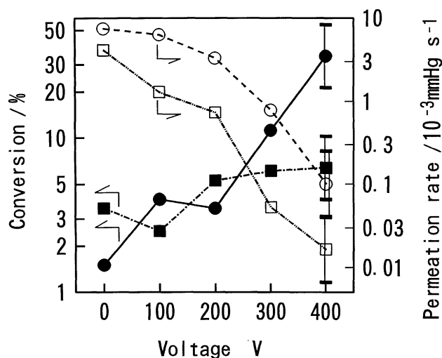
Figure 2. Conversion to n -butane (●) and t -2-butene (■) and permeation rates of \text{H}_2 (○) and c -2-butene (□) as a function of applied voltage at 20 mmHg. The outlet pressure: 0-0.2 mmHg.
