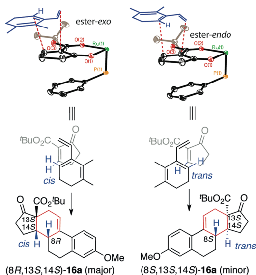
Figure 3. Sketches of the possible approaches of Dane's diene ( 15 ) to 7a . Part of the methoxybenzene ring of 15 is omitted for clarity.
