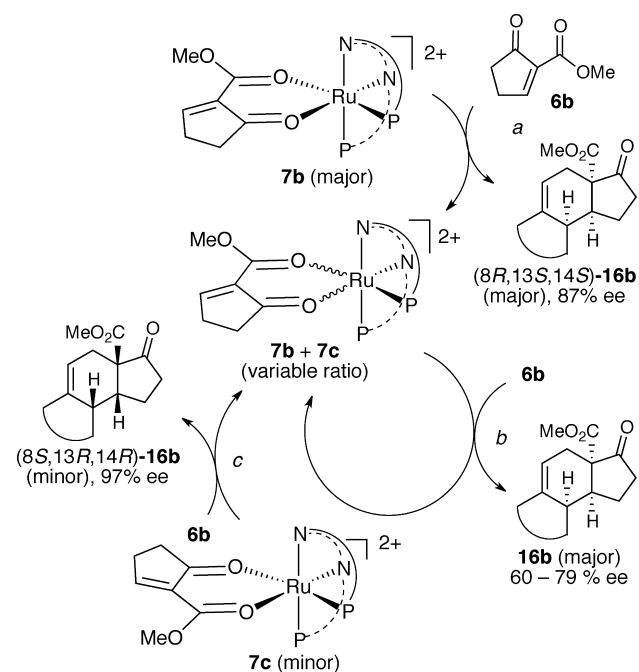
Scheme 7. General Stereochemical Course of the Catalytic Diels–Alder Reaction with 6b and 15
