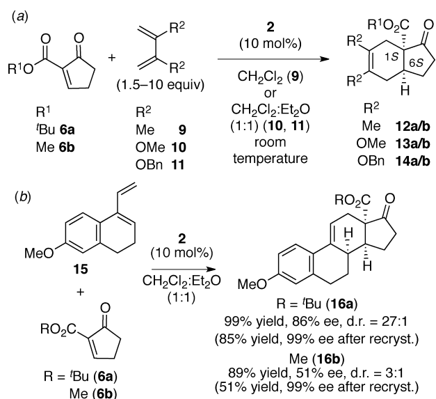
Scheme 2. Asymmetric Diels–Alder Reaction with Substituted 2,3-Butadienes
