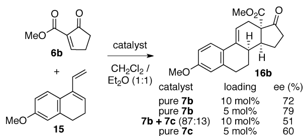
Scheme 6. Catalytic Reactions with Preformed Substrate/Catalyst Adducts 7b/7c
