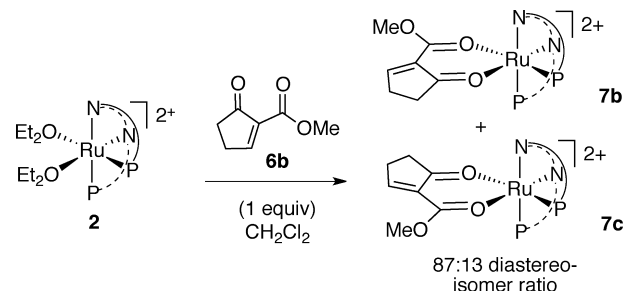
Scheme 5. Direct Synthesis of 7b/7c from 2 and 6b
