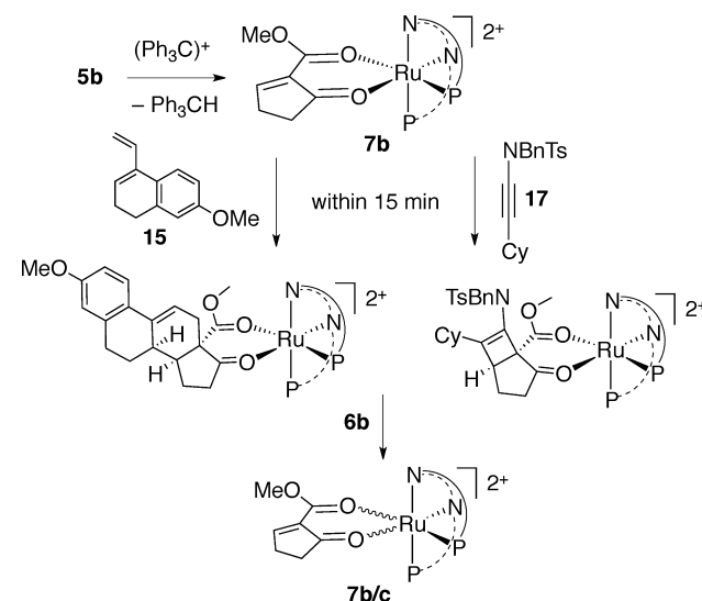
Scheme 8. Regeneration of the Substrate/Catalyst Adduct
