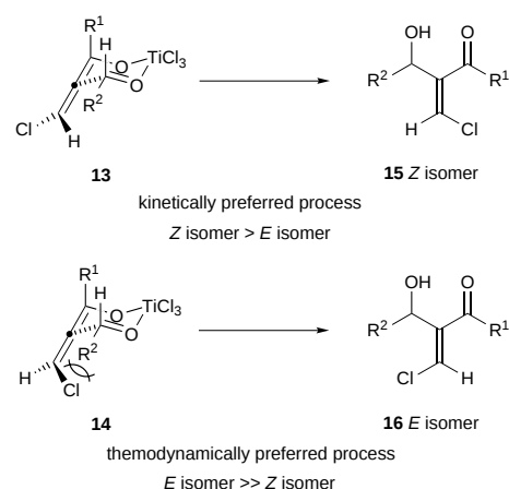
Scheme 2. Mechanism for formation of \alpha -(chloromethylene)aldols 15 and 16 .
