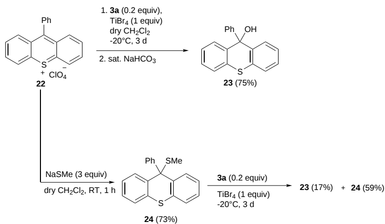
Scheme 4. Attempt to trap methanethiolate ion.
