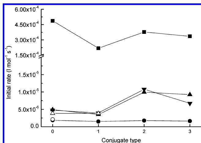
Figure 8. Correlation between the initial rate ( v_i ) for scavenging of DPPH • in aqueous micelles (pH 7.0) and type of conjugate for each antioxidant and its derivatives. A group (■): A0 (Trolox), A1, A2, and A3. B group (●): B0 (dihydroferulic acid), B1, B2, and B3. B0' (○) (ferulic acid). C group (▲): C0 (dihydrocaffeic acid), C1, C2, and C3. C' group (△): C0' (caffeic acid) and C1'. D group (▼): D0 (gallic acid), D1, D2, and D3.
