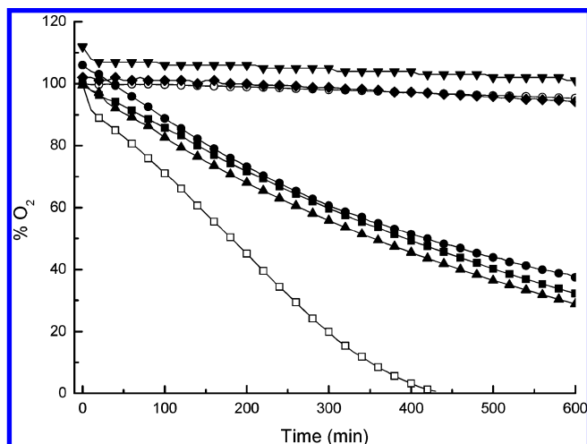
Figure 9. Oxygen consumption in an emulsion of methyl lineolate, Tween 20, and phosphate buffer (25 °C, pH 6.8) with initiation of oxidation by MMB in the presence of 7.9 \mu M of ferulic acid (●), dihydroferulic acid (■), B1 (▲), B2 (▼), and B3 (◆) in the absence of antioxidant (□) or both antioxidant and MMB (○).
