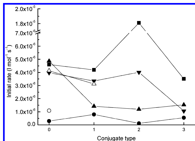
Figure 6. Correlation between the initial rate ( v_i ) for scavenging of DPPH • in MeOH and type of conjugate for each antioxidant and its derivatives. A group (■): A0 (Trolox), A1, A2, and A3. B group (●): B0 (dihydroferulic acid), B1, B2, and B3. B0' (○) (ferulic acid). C group (▲): C0 (dihydrocaffeic acid), C1, C2, and C3. C' group (△): C0' (caffeic acid) and C1'. D group (▼): D0 (gallic acid), D1, D2, and D3.
