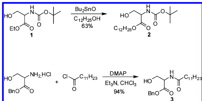
Figure 1. Synthesis of serine building blocks.
