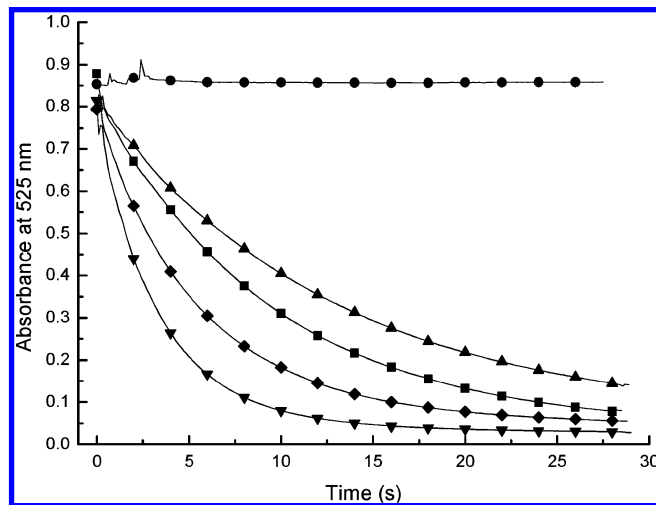
Figure 7. Scavenging of DPPH • (0.1 mM) in emulsion with 0.1 M sodium phosphate buffer (pH 7.0) and 4% (w/v) Tween 20 at 25 °C by 1.0 mM of gallic acid (■), D1 (▲), D2 (▼), and D3 (◆) and in absence of antioxidant (●).
