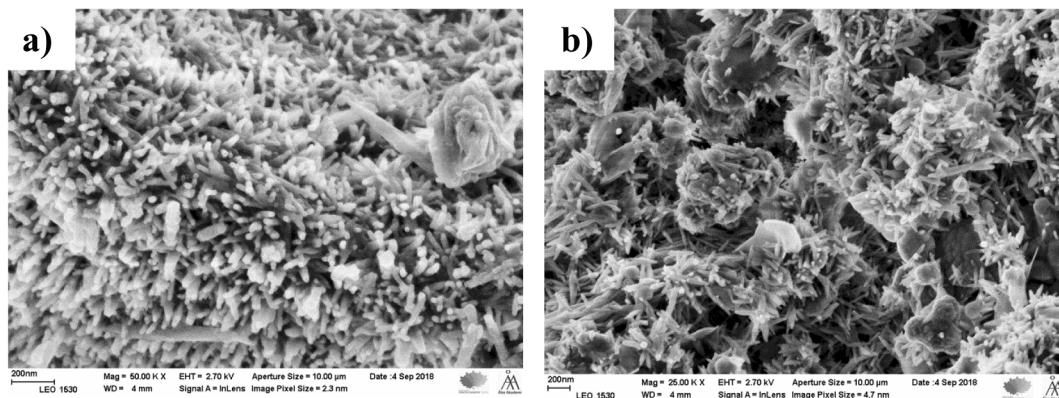
Fig. 3. SEM micrographs of slag catalytic materials synthesized via water treatment without an US step: a) st 48 h; b) rot 48 h, 150 °C.
