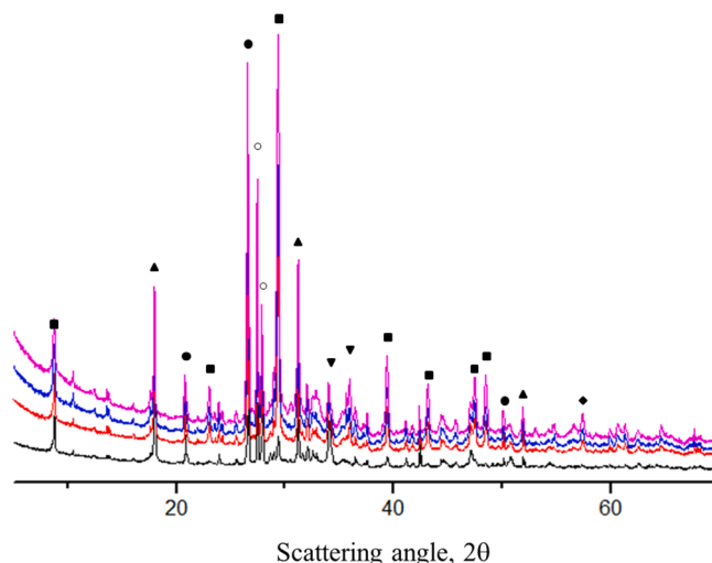
Fig. 13. XRD patterns of the raw material and materials obtained by alkaline treatment with 0.6 M NaOH. Notation: initial slag (black); NaOH US (50 W, 4 h) st 48 h (red); NaOH US (80 W, 4 h) st 48 h (dark blue); NaOH US (50 W, 4 h) rot 48 h, 150^\circ\text{C} (pink). Symbols: \text{SiO}_2 (●); \text{Al}_2\text{O}_3 (◆); \text{Fe}_2\text{O}_3 (▼); \text{TiO}_2 (○); \text{Ca}(\text{OH})_2 (▲); \text{CaCO}_3 (■). (For interpretation of the references to colour in this figure legend, the reader is referred to the web version of this article.)
