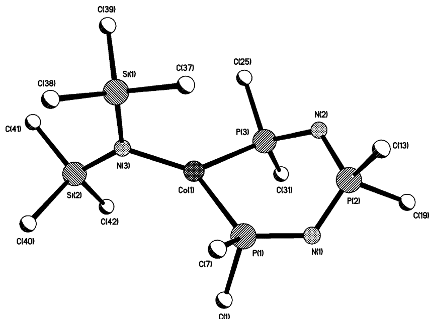
Figure 2. Molecular structure of 2 . Hydrogen atoms and Ph rings are omitted for clarity.
