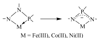
Figure 1. Molecular structure of 1 . Hydrogen atoms are omitted for clarity.
