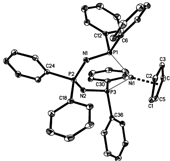
Figure 3. Molecular structure of 3 . Hydrogen atoms are omitted for clarity.
