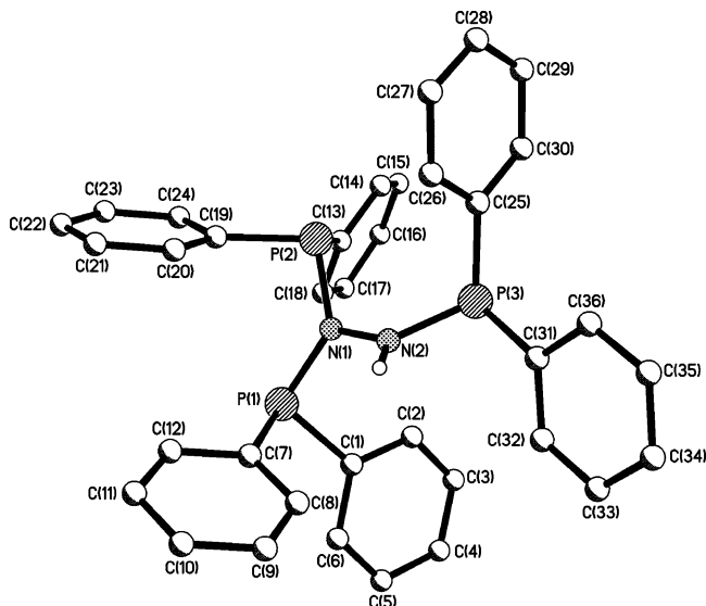
Figure 1. Molecular structure of 1 . Hydrogen atoms are omitted for clarity.
