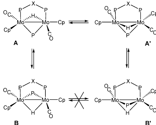
Scheme 1. Fluxional Process and Isomerization Equilibrium Proposed for Compounds 2a and 2c a
