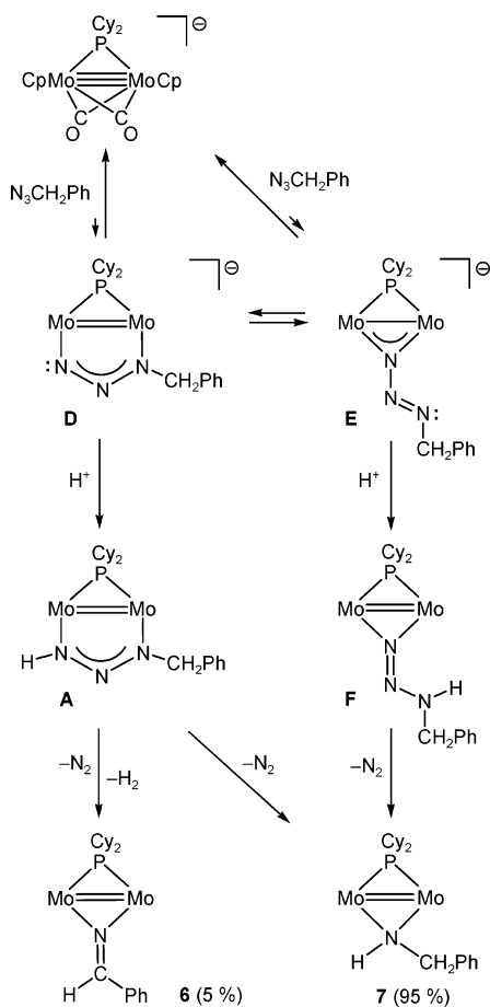
Scheme 4. Reaction Pathways Operative in the Reactions of the Anion [\text{Mo}_2\text{Cp}_2(\mu\text{-PCy}_2)(\mu\text{-CO})_2]^- with \text{PhCH}_2\text{N}_3 in the Presence of \text{H}_2\text{O}^a
