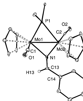
Figure 3. ORTEP diagram (30% probability) of compound 6 , with H atoms omitted, except the azavinylidene H atom, and Cy rings and t\text{Bu} groups omitted, except the corresponding \text{C}^1 atoms.
