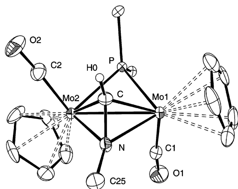
Figure 2. ORTEP diagram (30% probability) of compound 4b , 1 with H atoms omitted, except the formimidoyl H atom, and Cy rings and 'Bu groups omitted, except the corresponding C 1 atoms. Selected bond lengths (Å) and angles (deg): Mo(1)–Mo(2) = 2.883(2), Mo(1)–P = 2.416(2), Mo(2)–P = 2.436(2), Mo(1)–C(1) = 1.959(6), Mo(1)–C = 2.101(6), Mo(1)–N = 2.187(4), Mo(2)–C(2) = 1.914(6), Mo(2)–C = 2.115(6), Mo(2)–N = 2.157(4), C–N = 1.388(7); C(1)–Mo(1)–Mo(2) = 80.4(2), C(2)–Mo(2)–Mo(1) = 111.5(2), N–Mo(1)–P = 100.4(1), N–Mo(1)–P = 79.4(2).
