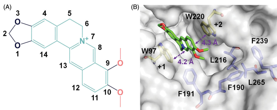
Figure 1. Crystal structure of SmChiB in complex with berberine. (A) Structure of berberine. The conjugate tetracycle plane is shown in green-cyan, the 9- O -methoxy and 10- O -methoxy moieties are shown in pink. (B) Binding mode of berberine in the active pocket of SmChiB . Berberine is shown in stick representation with carbon atoms in yellow. The amino residues forming the hydrophobic cavity extended near the +2 subsite are labelled and shown as stick representation with carbon atoms in blue. The numbers indicate the subsite to which the berberine is bound.
