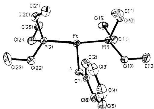
Figure 1. Thermal ellipsoid diagram (50%) and labeling scheme for PtH(NHPh)(PEt 3 ) 2 (I).
