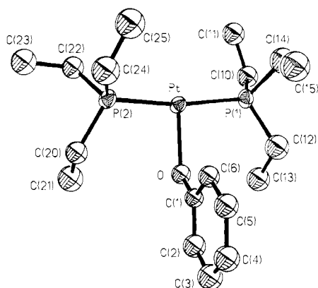
Figure 4. Thermal ellipsoid diagram (30%) and labeling scheme for \text{PtH}(\text{OPh})(\text{PEt}_3)_2 (II).
