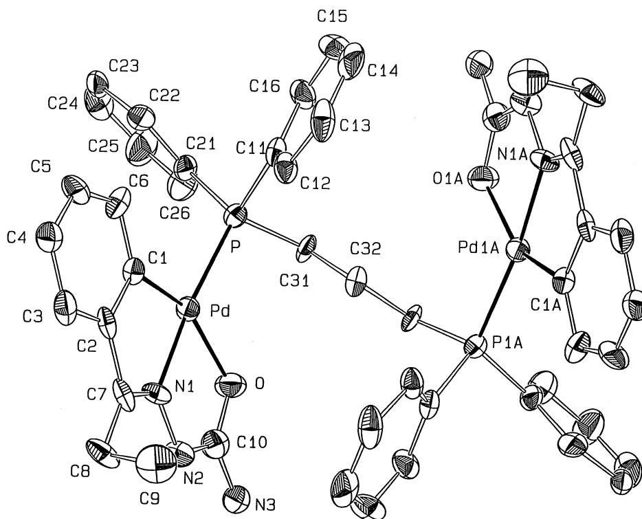
Fig. 1. Molecular structure of [\{Pd[C_6H_4C(Et)=NN(H)C(=O)NH_2\}2(\mu-Ph_2P-(CH_2)_3PPh_2)] [ClO_4]_2 .
