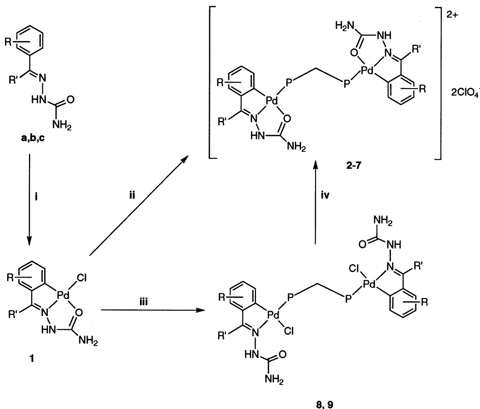
Scheme 1. Treatment of the semicarbazone ligands a , b or c with Li_2[PdCl_4] in methanol (i) gave compounds 1a–c , which were further reacted (ii) to give 2–7 or (iii) 8, 9 followed by (iv) resulting in 2–7 .
