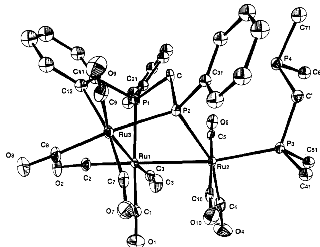
Figure 2. Perspective view of the complex Ru_3(CO)_9(\eta^1\text{-dppm})(\mu_3-\eta^3-P(C_6H_5)CH_2P(C_6H_5)(C_6H_4))(3c) . Only the ipso carbon atoms of the phenyl rings attached to atoms P(3) and P(4) are shown.
