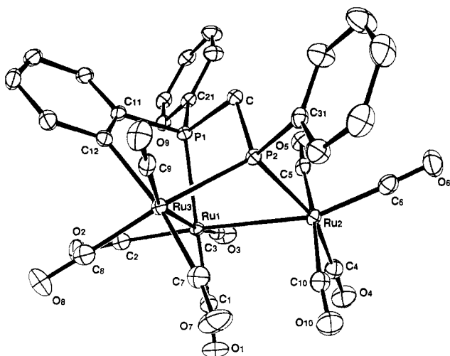
Figure 1. Perspective view of the complex Ru_3(CO)_{10}(\mu_3-\eta^3-P-(C_6H_5)CH_2P(C_6H_5)(C_6H_4))(3a) . Here and in Figures 2 and 3 vibrational ellipsoids are drawn at the 50% probability level.
