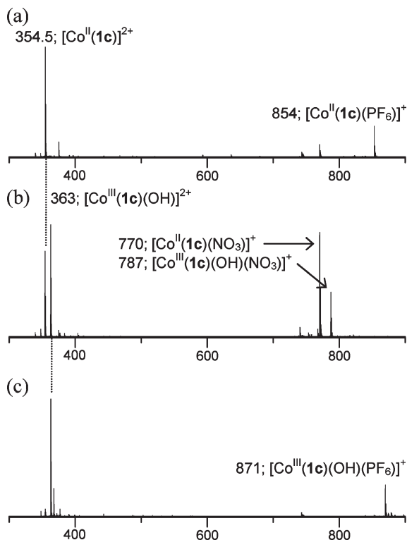
Figure 4. ESI-mass spectra of (a) 2c' , (b) after the exposure of 2c' to O_2 gas for 12 h, and (c) 2c'' .
