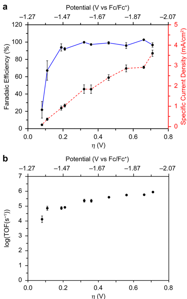
Figure 5. Electrochemical \text{CO}_2 reduction performance of [\text{Fe1}]^{2+} . (a) Selectivity of [\text{Fe1}]^{2+} for \text{CO}_2 reduction to CO at varying overpotentials and specific current densities for CO ( j_{\text{CO}} ) production (averages of three experiments). (b) Catalytic Tafel plot for [\text{Fe1}]^{2+} obtained from CPE experiments in acetonitrile with added phenol (3.5 M). CPE experiments were collected in an electrolyte of 0.10 M TBAPF 6 dissolved in \text{CH}_3\text{CN} .
