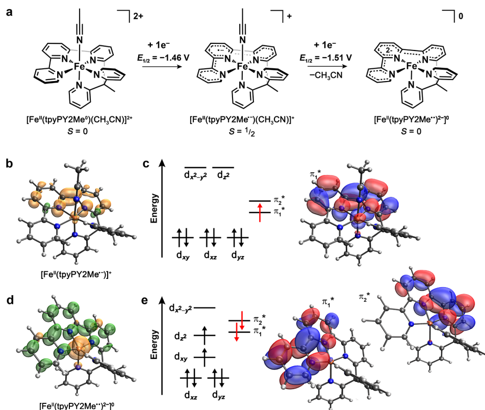
Figure 8. DFT analysis and calculated molecular orbitals for [FeI] + and [FeI] 0 species. (a) DFT predicted pathway for reduction of [FeI] 2+ to the open-shell singlet [FeI] 0 , [Fe(tpyPY2Me •• ) 2- ] 0 . The computed reduction potentials are given for reduction of [FeI] 2+ to [FeI] + and [FeI] + to [FeI] 0 . See Table S11 for the predicted reduction pathways for [Zn(1)] 2+/0 and for the closed-shell singlet [FeI] 0 , [Fe(tpyPY2Me) 2- ] 0 . (b) Spin density plot and (c) simplified molecular orbital diagram of the one electron reduced intermediate [FeI] + . (d) Spin density plot and (e) simplified molecular orbital diagram of [FeI] 0 ([Fe(tpyPY2Me •• ) 2- ] 0 ). Localized metal orbitals are depicted in the Supporting Information.
