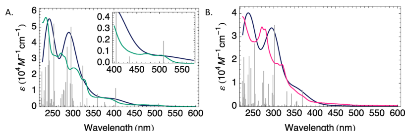
Figure 9. (A) Calculated (blue) and experimental (green) UV–vis absorption spectra for 2a . The region from 400 to 580 nm is enlarged in the inset to show that the weakest low energy transition is predicted by the calculations. (B) Calculated (blue) and experimental (pink) UV–vis absorption spectra for 3a . Calculated spectra were generated from Gaussian TD-DFT calculations using Gausssum software with fwhm = 4000 \text{cm}^{-1} . Calculated oscillator strengths are included as vertical lines.
