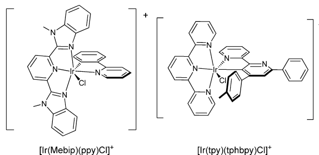
Figure 2. [\text{Ir}(\text{N}^{\wedge}\text{N}^{\wedge}\text{N})(\text{C}^{\wedge}\text{N})\text{L}]^+ type complexes previously reported by Obara et al. (left) 24 and Bexon et al. (right). 21
