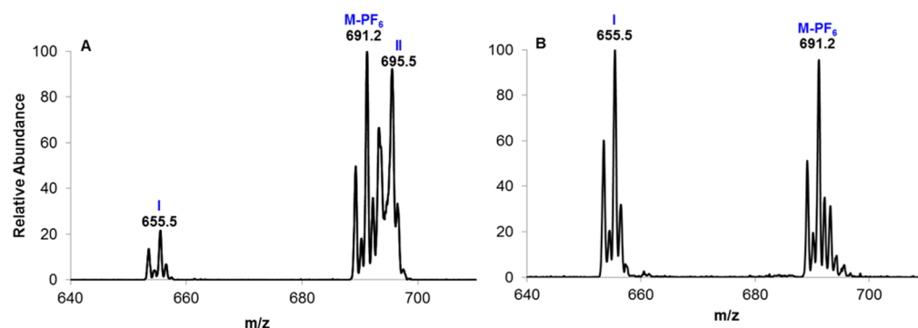
Figure 5. Electrospray ionization mass spectra collected for 2d in (A) acetonitrile and (B) methanol. Peak m/z values are given with black labels while assignments are made in blue. Spectra were collected with 50–60 \mu\text{M} solutions.
