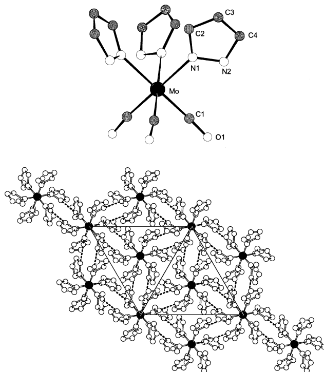
Fig. 1. Top: molecular drawing for [\text{Mo}(\text{CO})_3(\text{Hpz})_3] , with partial labeling scheme. Bottom: crystal packing, viewed down [001] , showing \text{N-H}\cdots\text{O} interactions (fragmented lines). Relevant bond distances ( \text{\AA} ) and angles ( ^\circ ), with estimated S.D.'s in parentheses: \text{Mo-N1} 2.317(9), \text{C1-Mo-C1'} 84.2(7), \text{N1-Mo-N1'} 83.5(6), cis - \text{C1-Mo-N1} 96.1(7), trans - \text{C1-Mo-N1} 179.5(1), \text{N-H}\cdots\text{O} 2.753, intermolecular \pi\cdots\pi interaction: \text{B}\cdots\text{B} 3.63 ( \text{B} = pyrazole center of mass).
