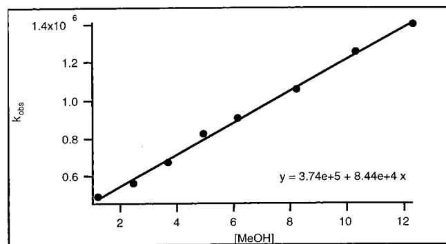
Figure 4. k_{obs} of decay of 1 vs [MeOH] in benzene at ambient temperature.
