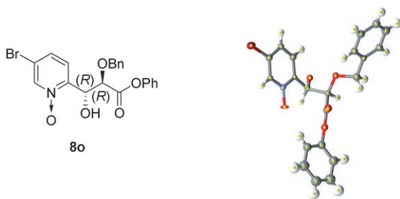
Figure 1. X-ray crystallographic structure of 8o .
