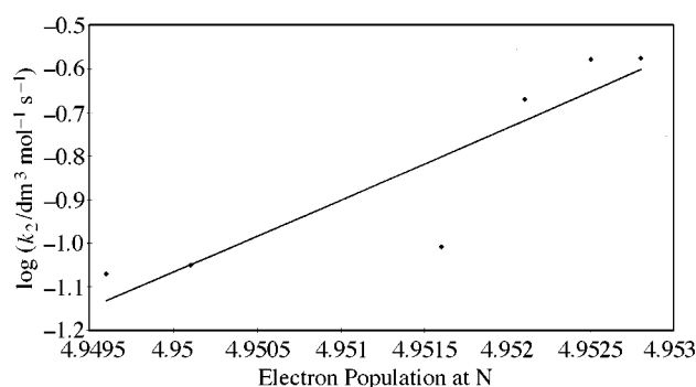
Fig. 4 Variation at 298 K of \log_{10}(k_2/\text{dm}^3 \text{ mol}^{-1} \text{ s}^{-1}) with electron population at nitroso N in p\text{-XC}_6\text{H}_4\text{NO} as calculated by the CNDO method
