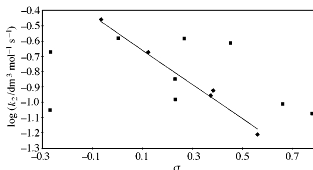
Fig. 3 Variation at 298 K of \log_{10}(k_2/\text{dm}^3 \text{mol}^{-1} \text{s}^{-1}) with Hammett \sigma constant of substituent X in \text{XC}_6\text{H}_4\text{NO} , p -X (■), m -X (◆)
