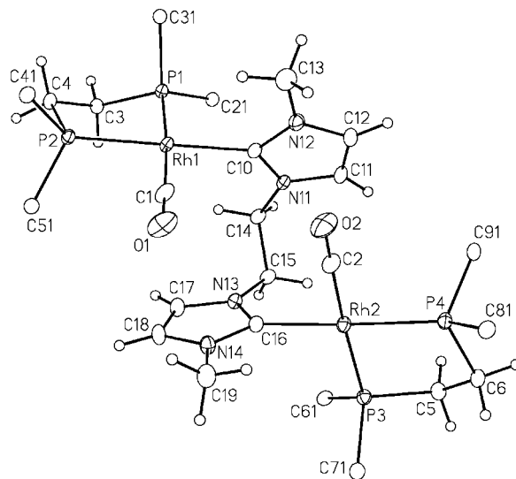
Figure 7. Representation of the complex dication of [Rh 2 (CO) 2 -(dppe) 2 (μ- R CC eth )] 2+ [CF 3 SO 3 ] 2 ( 8c ). Only the ipso carbons of the dppe phenyl rings are shown. Relevant parameters (distances in Å): Rh(1)–Rh(2) = 5.8605(6), Rh(1)–C(10) = 2.053(3), Rh(2)–C(16) = 2.069(3), Rh(1)–P(1) = 2.3185(7), Rh(1)–P(2) = 2.2796(7), Rh(2)–P(3) = 2.3246(7), Rh(2)–P(4) = 2.2763(7).
