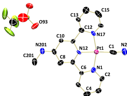
Figure 3. The molecular structure of a representative cation–anion pair of [\text{Pt}(\text{ma-T})\text{CN}]\text{OTf} \cdot \text{MeCN} with thermal ellipsoids set at 50% probability. Selected bond lengths (Å) and angles (deg) associated with the metal center: N1–Pt1 2.037(15), N12–Pt1 1.961(12), N17–Pt1 2.090(15), Pt1–C1 1.87(2); C1–N2 1.26(2); N1–Pt1–N12 78.8(5), N12–Pt1–C1 177.1(6), N1–Pt1–C1 98.4(6), N1–Pt1–N17 160.9(5), N12–Pt1–N17 82.1(5), N17–Pt1–C1 100.7(6); N2–C1–Pt1 175.3(15).
