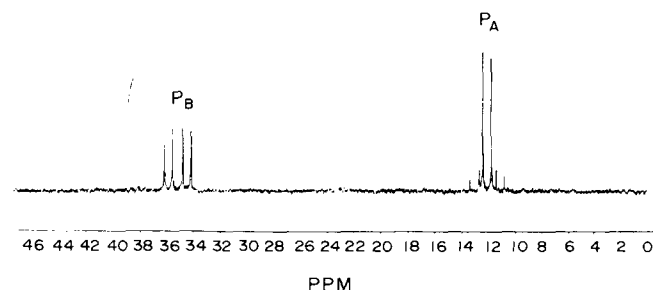
Fig. 2. 31 P-NMR spectrum of [(\text{CO})_2(\text{bpy})\text{W}(\mu\text{-CO})(\mu\text{-dppm})\text{RhCl}(\text{NBD})] .
