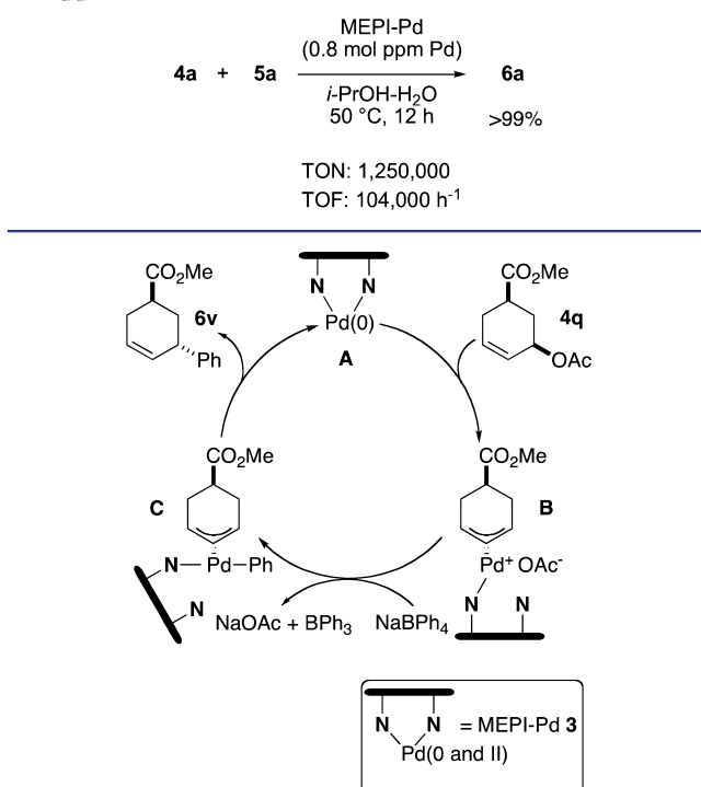
Figure 4. Plausible catalytic cycle of allylic arylation of 4q with 5a.
