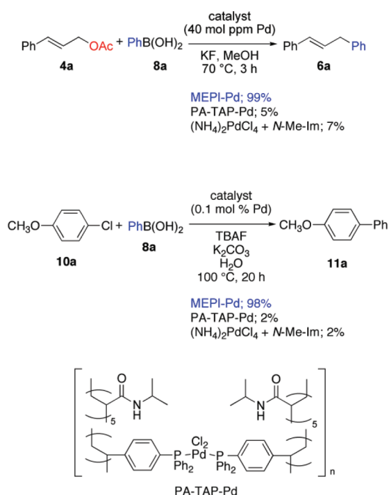
Scheme 6. MEPI-Pd vs PA-TAP-Pd and [(\text{NH}_4)_2\text{PdCl}_4 + N\text{-Me-imdazole}]
