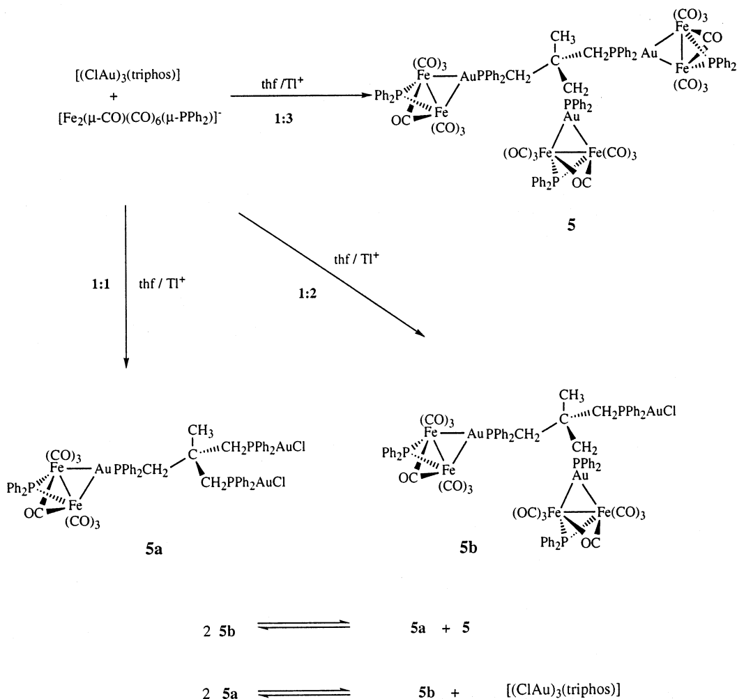
Scheme 3. Reaction of [\text{Fe}_2(\mu\text{-CO})(\text{CO})_6(\mu\text{-PPh}_2)]^- with [(\text{ClAu})_3(\text{triphos})] , leading to the formation of ( 5 ), ( 5a ) and ( 5b ), depending on the concentration of gold compound used.
