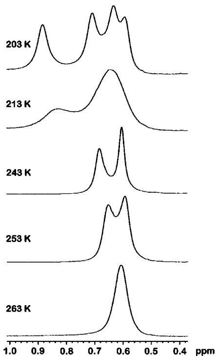
Figure 5. Variable-temperature ^1\text{H} NMR spectra of [(\text{CH}_3\text{OCH}_2\text{CH}_2)_2\text{NCH}_2\text{-C}_6\text{H}_2\text{-3,5-(CMe}_3)_2\text{-2-O}]\text{Y}(\text{CH}_2\text{SiMe}_2\text{Ph})_2 ( 7a ) showing the \text{Si}(\text{CH}_3)_2\text{Ph} peaks (toluene- d_8 , 500 MHz).
