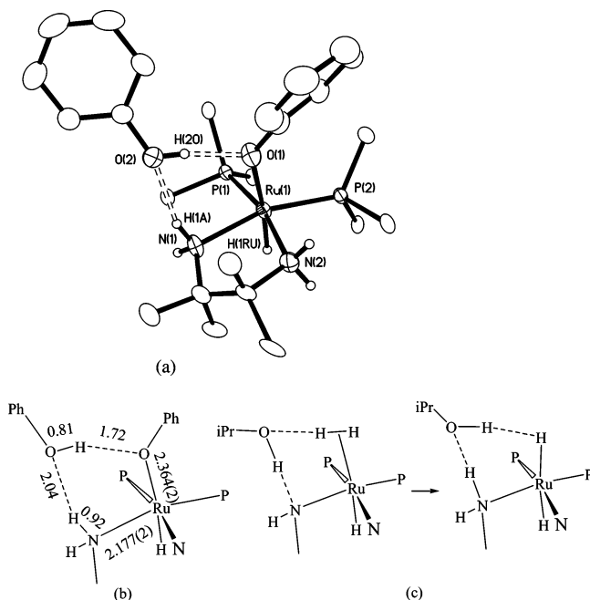
Figure 2. (a) Molecular structure of \text{RuH(OPh)(tmen)(PPh}_3)_2 \cdot \text{HOPh} . Selected bond distances (Å) and angles (deg): \text{Ru(1)–O(1)} = 2.364(2) , \text{Ru(1)–H(1RU)} = 1.53(3) , \text{Ru(1)–N(1)} = 2.177(2) , \text{Ru(1)–N(2)} = 2.179(2) , \text{Ru(1)–P(2)} = 2.2690(7) , \text{Ru(1)–P(1)} = 2.2697(8) ; \text{H(1RU)–Ru(1)–N(1)} = 88(1) , \text{N(1)–Ru(1)–N(2)} = 75.20(9) , \text{N(1)–Ru(1)–P(2)} = 163.57(7) , \text{N(2)–Ru(1)–P(2)} = 92.01(7) , \text{N(1)–Ru(1)–P(1)} = 93.13(7) , \text{N(2)–Ru(1)–P(1)} = 167.31(7) , \text{P(2)–Ru(1)–P(1)} = 98.49(3) , \text{N(1)–Ru(1)–O(1)} = 83.83(8) , \text{N(2)–Ru(1)–O(1)} = 80.87(9) , \text{P(2)–Ru(1)–O(1)} = 104.62(5) , \text{P(1)–Ru(1)–O(1)} = 103.14(6) . (b) The six-membered ring. (c) Related ring structures proposed for the alcohol-assisted splitting of dihydrogen.
