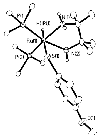
Figure 3. Molecular structure of \text{RuH(4-SC}_6\text{H}_4\text{OMe)(tmen)(PPh}_3)_2 . Selected bond distances (Å) and angles (deg): \text{Ru(1)–H(1RU)} = 1.57(3) , \text{Ru(1)–N(1)} = 2.181(2) , \text{Ru(1)–N(2)} = 2.205(2) , \text{Ru(1)–P(1)} = 2.2695(8) , \text{Ru(1)–P(2)} = 2.2715(9) , \text{Ru(1)–S(1)} = 2.5274(9) ; \text{N(1)–Ru(1)–N(2)} = 73.54(9) , \text{N(1)–Ru(1)–P(1)} = 92.05(7) , \text{N(2)–Ru(1)–P(1)} = 165.54(7) , \text{N(1)–Ru(1)–P(2)} = 163.66(7) , \text{N(2)–Ru(1)–P(2)} = 94.46(7) , \text{P(1)–Ru(1)–P(2)} = 99.46(3) , \text{N(1)–Ru(1)–S(1)} = 84.12(7) , \text{N(2)–Ru(1)–S(1)} = 88.24(7) , \text{P(1)–Ru(1)–S(1)} = 91.41(3) , \text{P(2)–Ru(1)–S(1)} = 106.99(3) .
