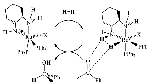
Scheme 2. Hypothetical Cycle for the Hydrogenation of Acetophenone Catalyzed by the Complexes \text{RuHX}(\text{dach})(\text{PPh}_3)_2 with X Trans to H a
