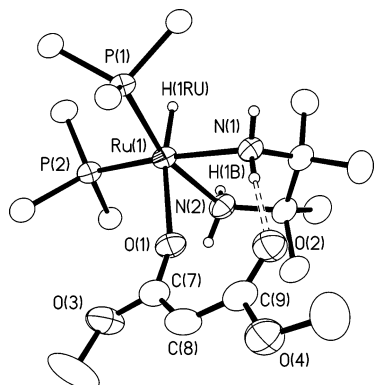
Figure 6. Molecular structure of RuH(CH(COOEt) 2 )(tmen)(PPh 3 ) 2 . Selected bond distances (Å) and angles (deg): Ru(1)–H(1RU) = 1.50, Ru(1)–N(1) = 2.154(3), Ru(1)–N(2) = 2.180(3), Ru(1)–P(2) = 2.2392(9), Ru(1)–P(1) = 2.2494(8), Ru(1)–O(1) = 2.265(2); N(1)–Ru(1)–N(2) = 75.6(1), N(1)–Ru(1)–P(2) = 170.26(7), N(2)–Ru(1)–P(2) = 94.72(8), N(1)–Ru(1)–P(1) = 91.85(7), N(2)–Ru(1)–P(1) = 163.82(8), P(2)–Ru(1)–P(1) = 97.35(3), N(1)–Ru(1)–O(1) = 77.3(1), N(2)–Ru(1)–O(1) = 78.9(1), P(2)–Ru(1)–O(1) = 102.61(7), P(1)–Ru(1)–O(1) = 108.70(7).
