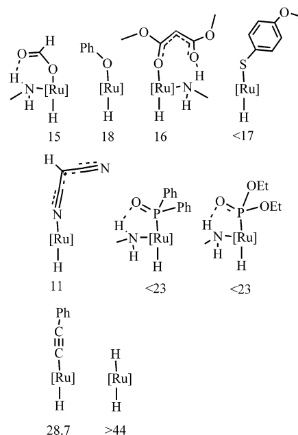
Chart 1. Coordination Mode of the X Ligand in the Complex \text{trans-RuHX}(\text{diamine})(\text{PPh}_3)_2 Arranged by the Group in the Periodic Table of the Atom Attached to Ruthenium and the \text{pK}_a^{\text{DMSO}} Values of the Weak Acid HX Used To Generate the Complex According to Eq 1 or 2
