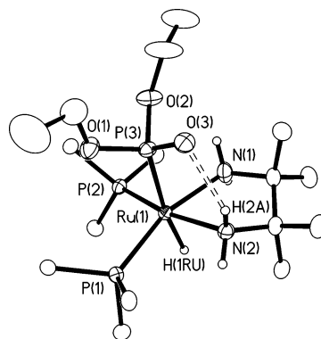
Figure 4. Molecular structure of \text{RuH(OP(OEt)}_2\text{)(tmen)(PPh}_3)_2 . Selected bond distances (Å) and angles (deg): \text{Ru(1)–H(1RU)} = 1.63(3) , \text{Ru(1)–N(1)} = 2.166(2) , \text{Ru(1)–N(2)} = 2.181(2) , \text{Ru(1)–P(1)} = 2.2772(5) , \text{Ru(1)–P(2)} = 2.2872(5) , \text{Ru(1)–P(3)} = 2.3486(5) ; \text{H(1RU)–Ru(1)–N(1)} = 82.0(9) , \text{H(1RU)–Ru(1)–N(2)} = 91.6(9) , \text{N(1)–Ru(1)–N(2)} = 75.19(7) , \text{H(1RU)–Ru(1)–P(1)} = 86.4(9) , \text{N(1)–Ru(1)–P(1)} = 163.52(5) , \text{N(2)–Ru(1)–P(1)} = 93.50(5) , \text{H(1RU)–Ru(1)–P(2)} = 85.0(9) , \text{N(1)–Ru(1)–P(2)} = 92.27(5) , \text{N(2)–Ru(1)–P(2)} = 167.37(5) , \text{P(1)–Ru(1)–P(2)} = 98.42(2) , \text{H(1RU)–Ru(1)–P(3)} = 171.7(9) , \text{N(1)–Ru(1)–P(3)} = 90.03(6) , \text{N(2)–Ru(1)–P(3)} = 83.79(5) , \text{P(1)–Ru(1)–P(3)} = 100.79(2) , \text{P(2)–Ru(1)–P(3)} = 97.98(2) .
