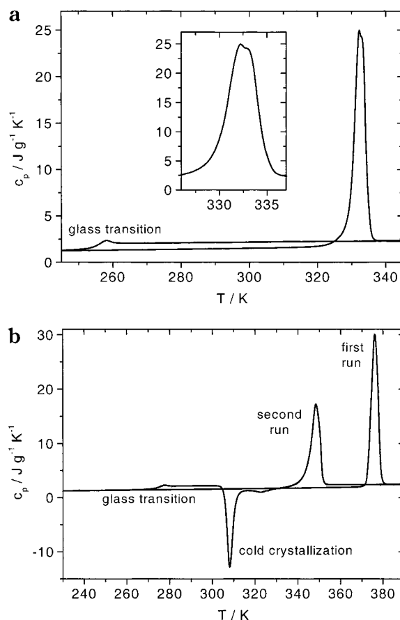
Figure 3. (a) First and second heating of 4- tert -butylcatechol. Heating rate 10 K·min -1 . The inset shows a magnified part of the melting peak. (b) First and second heating of 3,5-di- tert -butylcatechol. Heating rate 10 K·min -1 .
