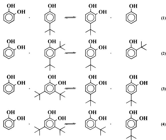
Figure 1. Equilibrium reactions of transalkylation of tert -butylcatechols and tert -butylphenols in the liquid phase.
