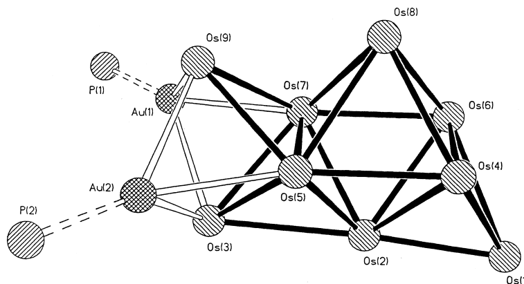
Fig. 4. Diagram depicting metal core geometry of [\text{Os}_9(\text{CO})_{24}\{\text{Au}(\text{PCy}_3)\}_2] ( 2b ).
