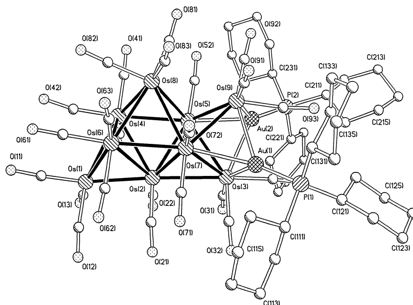
Fig. 3. Diagram depicting molecular structure of [\text{Os}_9(\text{CO})_{24}\{\text{Au}(\text{PCy}_3)\}_2] ( 2b ).
