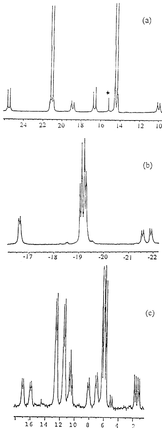
Fig. 1. ^{31}\text{P}\{^1\text{H}\} -NMR spectra (202.5 MHz) of: (a) cis,cis -[( p - \text{MeC}_6\text{H}_4 ) _2\text{Pt}(\mu\text{-SMe}_2)(\mu\text{-dppm})\text{Pt}\{(\text{CH}_2)_4\} ] ( 2b ); (b) [\text{Me}_3\text{Pt}(\mu\text{-I})(\mu\text{-dppm})\text{Pt}\{(\text{CH}_2)_4\}\text{Me}] ( 3b ); and (c) [\text{Me}_2\text{Pt}(\mu\text{-dppm})_2\text{Pt}\{(\text{CH}_2)_4\}] ( 6b ) at -60 °C.
