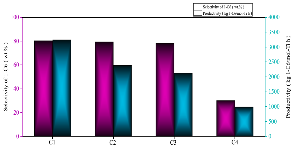
Fig. 6. Effect of various bridges on catalyst productivity; Al/Ti= 2000, time= 30 min, rpm= 600, solvent= toluene (20 mL), catalyst concentration= 1.5 \mu mol, temperature= 40 ^{\circ} C, ethylene pressure= 8 bar
