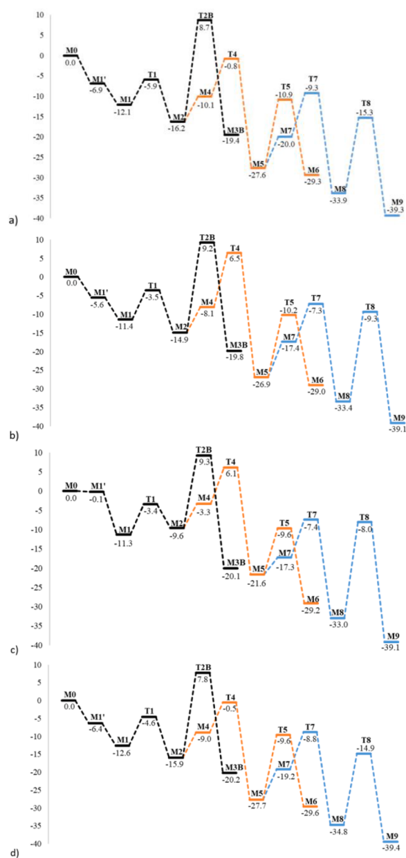
Fig. 7. Gibbs free energy profile (kcal·mol -1 ) for the ethylene oligomerization by catalysts (a) C1, (b) C2, (c) C3 and (d) C4, relative to compound M0 and considering toluene as a solvent.
