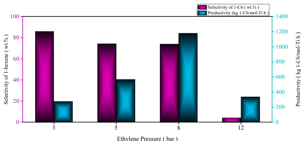
Fig. 4. Effect of ethylene pressure on catalyst productivity; Al/Ti= 2000, time= 30 min, rpm= 600, solvent = toluene (20 mL), catalyst (C2) concentration= 1.5 \mu mol, temperature= 20 °C
