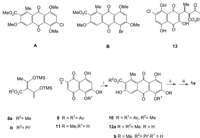
Scheme 3. For 1a and 1b . Reagents and conditions : 9 (i) toluene, 8a heat, 24 h, column chromatography, \text{SiO}_2 ; (ii) MeOH, 1% \text{Na}_2\text{CO}_3 ; (iii) HOAc–HCl, heat; (iv) for 1c , DMS, \text{Me}_2\text{CO} , \text{K}_2\text{CO}_3 , heat. Compound 11 from 3 , with \text{BF}_3 \cdot \text{MeOH} ; toluene, 8 , heat, column chromatography \text{SiO}_2 .
