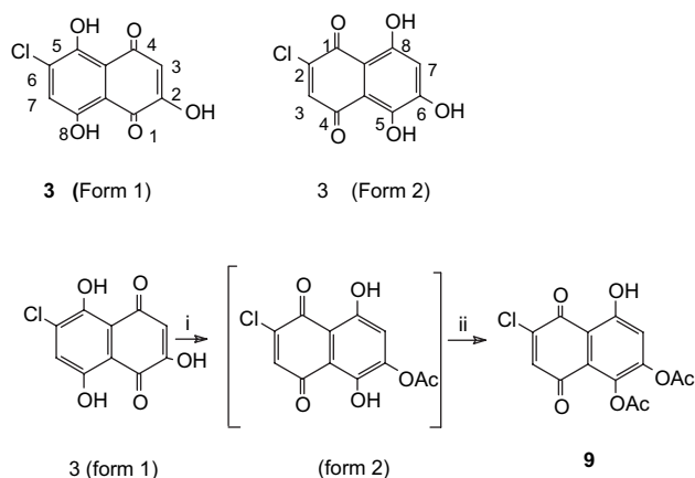
Scheme 2. Reagents and conditions: (i) \text{Ac}_2\text{O} , 100 °C, 3 h; (ii) vacuum to dryness.
