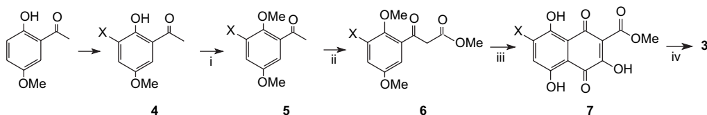
Scheme 1. Reagents and conditions: 4 ( \text{X}=\text{Cl} ) (i) NCS, HOAc, \text{Mg}(\text{OAc})_2 , rt, 24 h; DMS, \text{Me}_2\text{CO} , \text{K}_2\text{CO}_3 , heat, 24 h; (ii) NaOMe, MeOH, (\text{MeO})_2\text{CO} , heat; (iii) (\text{COCl})_2 , \text{MeNO}_2 , \text{AlCl}_3 , 0–80 °C, 3 h; (iv) 10% concd HCl–HOAc, 100 °C, 5 h.
