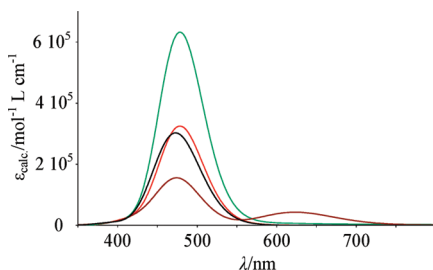
Figure 9. Theoretical absorption spectra from TDDFT calculations for \text{Ru}^{\text{II}} complexes. Ru-1 (red line), Ru-1' (brown line), Ru-2 (green line), Ru-3 (black line).
