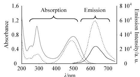
Figure 4. Absorption and emission spectra of L 3 (dotted lines) and Ru-3 (full lines), at 298 K in acetonitrile.
