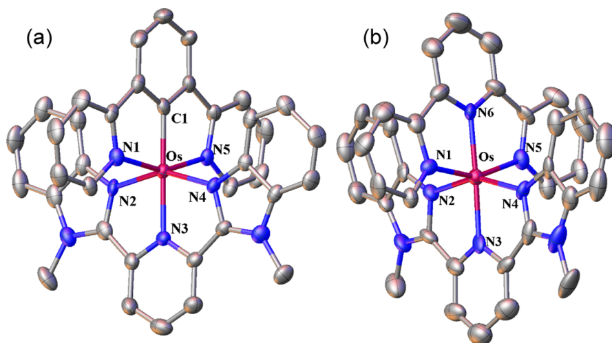
Figure 1. Thermal ellipsoid plots of the X-ray structures of (a) 2(\text{PF}_6) and (b) 6(\text{PF}_6)_2 with 30% probability. Counter anions and hydrogen atoms are omitted for clarity. Atom color code: carbon, gray; nitrogen, blue; osmium, brown.
