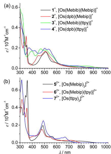
Figure 5. UV/vis absorption spectra of (a) cyclometalated complexes 1^+ to 4(\text{PF}_6)_2 and (b) noncyclometalated complexes 5(\text{PF}_6)_2 to 7(\text{PF}_6)_2 in \text{CH}_3\text{CN} . Anions are omitted for the complex labels for clarity.
