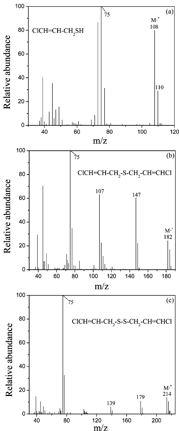
Figure 6. Mass spectra (EI) of transformation products obtained from the reaction of 1,3-D with HS - : (a) mercaptan (RSH), (b) thioether (RSR), and (c) disulfide product (RSSR).
