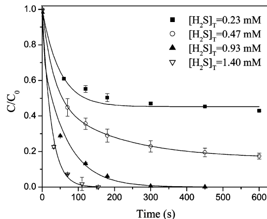
Figure 2. Example time courses for dissipation of chloropicrin in different initial ( \text{H}_2\text{S} ) T concentration solutions at constant temperature ( 21 \pm 0.5 °C) and approximately constant pH ( 6.9 \pm 0.1 ). C_0 is the initial concentration of chloropicrin (0.5 mM) in the solutions.
