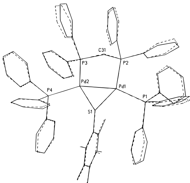
Figure 5. Fit of the two crystallographically independent cations in compound 5c (mean deviation for \text{SPd}_2\text{P}_2\text{C} = 0.027 Å).
