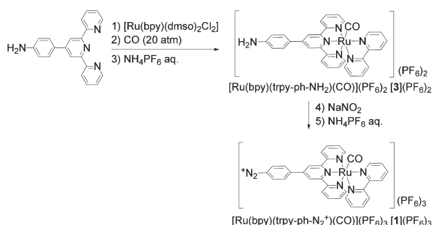
Scheme 1. Synthesis of diazonium ruthenium complex [1] (PF 6 ) 3 .
