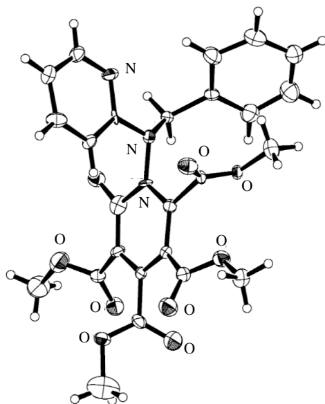
Figure 2. ORTEP view of pyridone detivative ( 6a )
