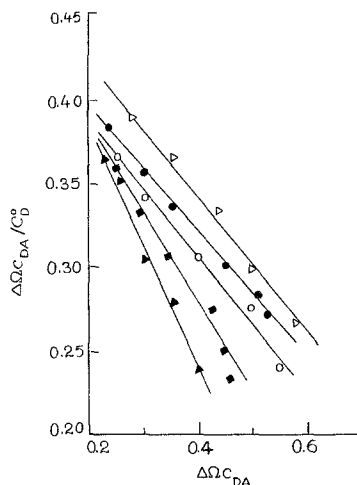
Fig. 1. Plot of \Delta\Omega C_{DA} vs. \Delta\Omega C_{DA}/C_D^\circ for indole-DDT ( \circ-\circ-\circ ), 2-methylindole-DDT ( \bullet-\bullet-\bullet ), 3-methylindole-DDT ( \Delta-\Delta-\Delta ), naphthalene-DDT ( \blacktriangle-\blacktriangle-\blacktriangle ) and benzene-DDT ( \blacksquare-\blacksquare-\blacksquare ) in \text{CCl}_4 at 30^\circ\text{C}
