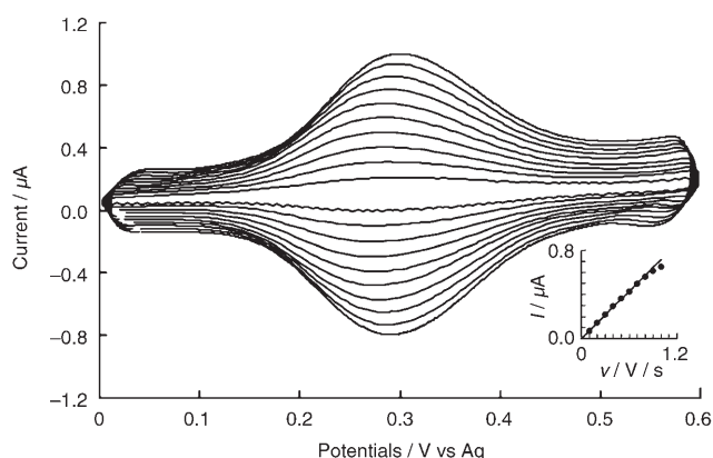
Figure 6. Cyclic voltammetry for Ir-C 18 on HOPG. a) Scan rate dependent cyclic voltammograms (0.1–1 \text{Vs}^{-1} ). b) Relationship between the peak current values and scan rates.
