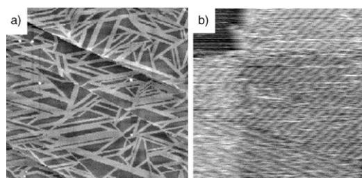
Figure 7. Samples of \text{Ir-C}_{18} on HOPG, annealed at 125^\circ\text{C} for 40 min. a) DFM image ( 5 \times 5 \mu\text{m}^2 ). b) STM image ( 100 \times 100 \text{ nm}^2 ; I = 3 \text{ pA} ; V = -1.0 \text{ V} ).
