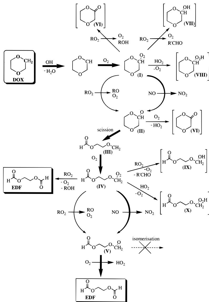
Figure 6. Mechanism for the OH-radical-initiated oxidation of 1,4-dioxane (DOX) depicting possible reaction channels both with and without the presence of \text{NO}_x . The reactions dominating under most atmospheric conditions showing arrows with bold type.
