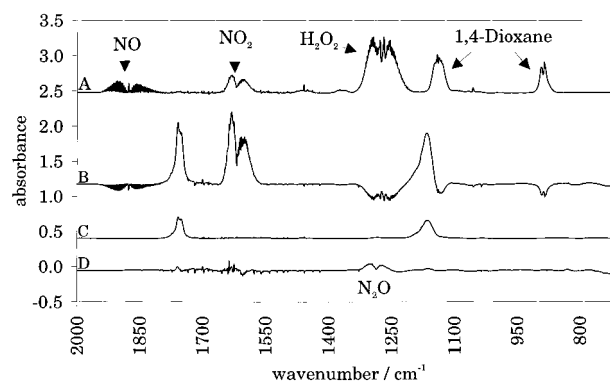
Figure 2. Infrared spectra recorded for a \text{H}_2\text{O}_2/\text{NO}_x/\text{DOX} photolysis system in the wavenumber region 2000\text{--}700 \text{ cm}^{-1} . Spectrum A was recorded before irradiation, B is a difference spectrum derived from a spectrum recorded after 10 min irradiation minus spectrum A, C is a reference spectrum of EDF, and D is the residual spectrum obtained after 10 min irradiation and subtraction of DOX and all identified products. The \text{N}_2\text{O} is introduced into the chamber as impurity with NO.
