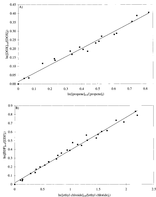
Figure 1. Kinetic data plotted according to eq 1 for reaction of (A) OH radicals with 1,4-dioxane (DOX) and (B) Cl atoms with ethylene glycol diformate (EDF).
