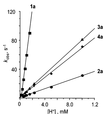
Figure 1. Dependence of the pseudo-first-order rate constants ( k_{\text{obs}}/\text{s}^{-1} ) on proton concentration for reactions of cis -[PtMe 2 L 2 ] complexes ( 1a – 4a , eq 2) in methanol at 298.2 K. For the sake of clarity the diagrams for compounds 5a – 8a have been omitted.
