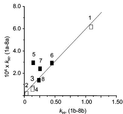
Figure 4. Correlation between the second-order rate constants k_{\text{H}} (M −1 s −1 ) for protonolysis of the dialkyl complexes cis -[PtMe 2 L 2 ] ( 1a–8a ) and related monoalkyl compounds cis -[PtMeClL 2 ] ( 1b–8b ) in methanol at 298 K. Numbers refer to compounds as listed in Table 3.
