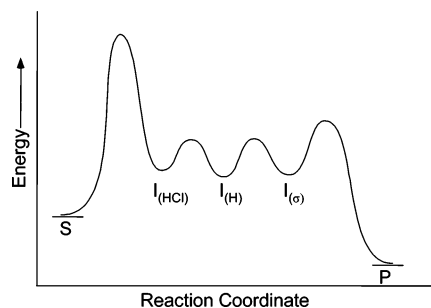
Figure 5. Qualitative coordinate reaction diagram for a rate-determining initial protonation in an S_E(\text{ox}) mechanism. The symbols S, I_{(\text{HCl})} , I_{(\text{H})} , and I_{(\sigma)} and P have the same meaning as in Figure 3.
