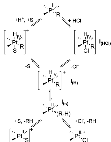
Scheme 3. Currently Accepted Oxidative-Addition–Reductive-Elimination Mechanism
