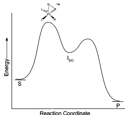
Figure 6. Qualitative coordinate reaction diagram for a rate-determining proton attack at the Pt–C \sigma -bond of S with release of alkane in a three-center transition state ( S_E2 mechanism).
