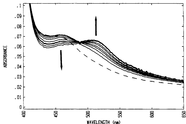
Figure 2. Electronic absorption spectra of a poly[ \text{Ru}(\text{Me}_4\text{bpy})_2(\text{vpy})_2 ] ^{2+} film ( \Gamma_{\text{Ru}} = 6.8 \times 10^{-9} mol/cm ^2 ) at various times over a photolysis (460-nm) period of 58 min. The external solution was 0.1 M aqueous \text{dmte}^- . The dashed line (---) shows the initial spectrum.
