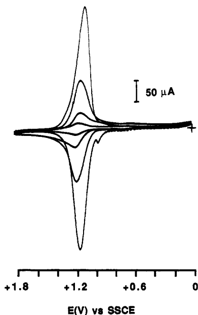
Figure 1. Cyclic voltammograms recorded in 0.1 M N(n\text{-Bu})_4\text{PF}_6/\text{CH}_3\text{CN} for a poly[ \text{Ru}(\text{Me}_4\text{bpy})_2(\text{vpy})_2 ] ^{2+} film following photolysis at 436 nm: I^0 = 1.17 einsteins/s \cdot\text{cm}^2 ; scan rate = 100 mV/s. Voltammograms were recorded at t = 0, 10, 18 , and 31 s. Each of the scans shown was recorded after an initial "conditioning" cycle.
