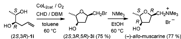
Scheme 2. Synthesis of (–)- allo -Muscarine
