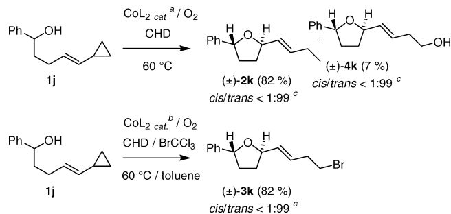
Scheme 3. Formation of Butenyl-Substituted Tetrahydrofurans
