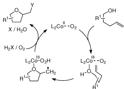
Scheme 1. Proposed Catalytic Cycle for Aerobic Alkenol Oxidation a
