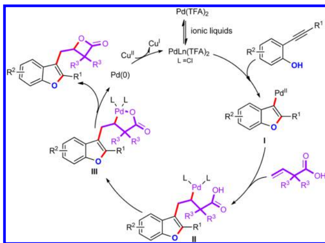
Scheme 6. Proposed Mechanism
