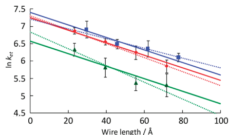
Figure 2. Plots of \ln(k_{\text{et}}) vs d for [\text{A}^x(\text{FeL})_{n-1}\text{FeT}] (blue, x = 1 ; green, x = 2 ; red, x = 3 ). Dashed lines were obtained by least-squares fitting for each x and solid lines by fitting for all x assuming the same slope.
